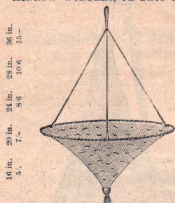
DOUBLE FOLDING MINNOW TRAP.
